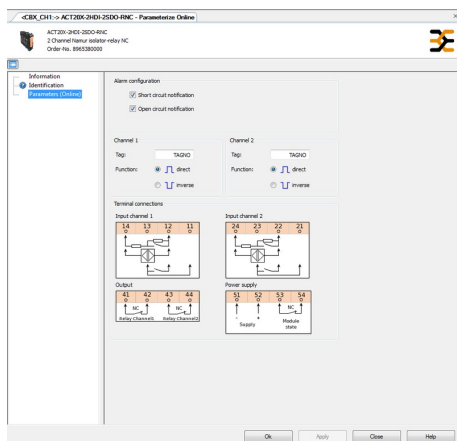
Screenshot of configuration with FDT/DTM software
