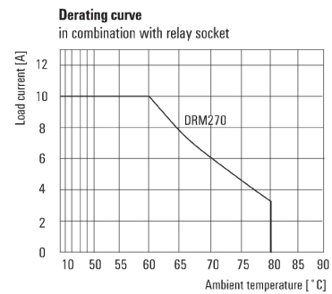
Relay in combination with base
