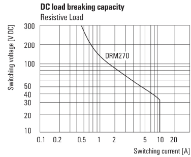
Resistive load
